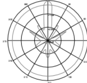
Vertical Pattern
